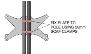
DOUBLE POLE MOUNT
